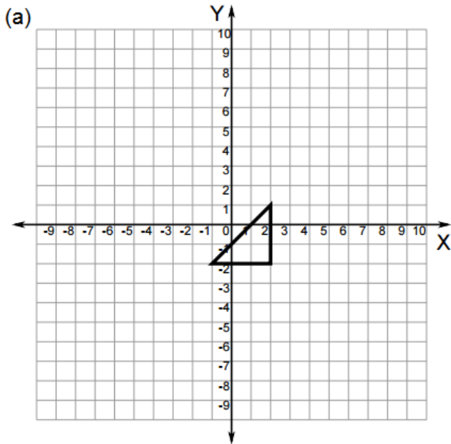
Enlarge with a scale factor of 3, centered at the origin.
