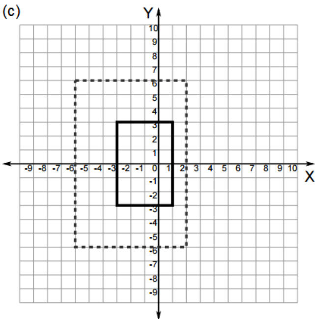
Enlarge with a scale factor of 2, centered at the origin.
